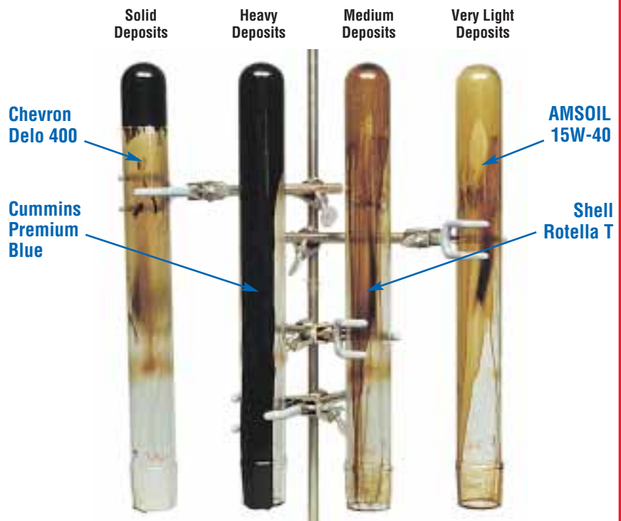
This severe high temperature deposit test shows AMSOIL Synthetic 15W-40 Heavy Duty Diesel and Marine Oil keeps engines cleaner longer than other major brand diesel oils do.
